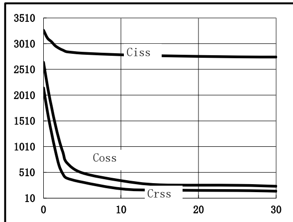
Fig.4 Capacitance Characteristics
